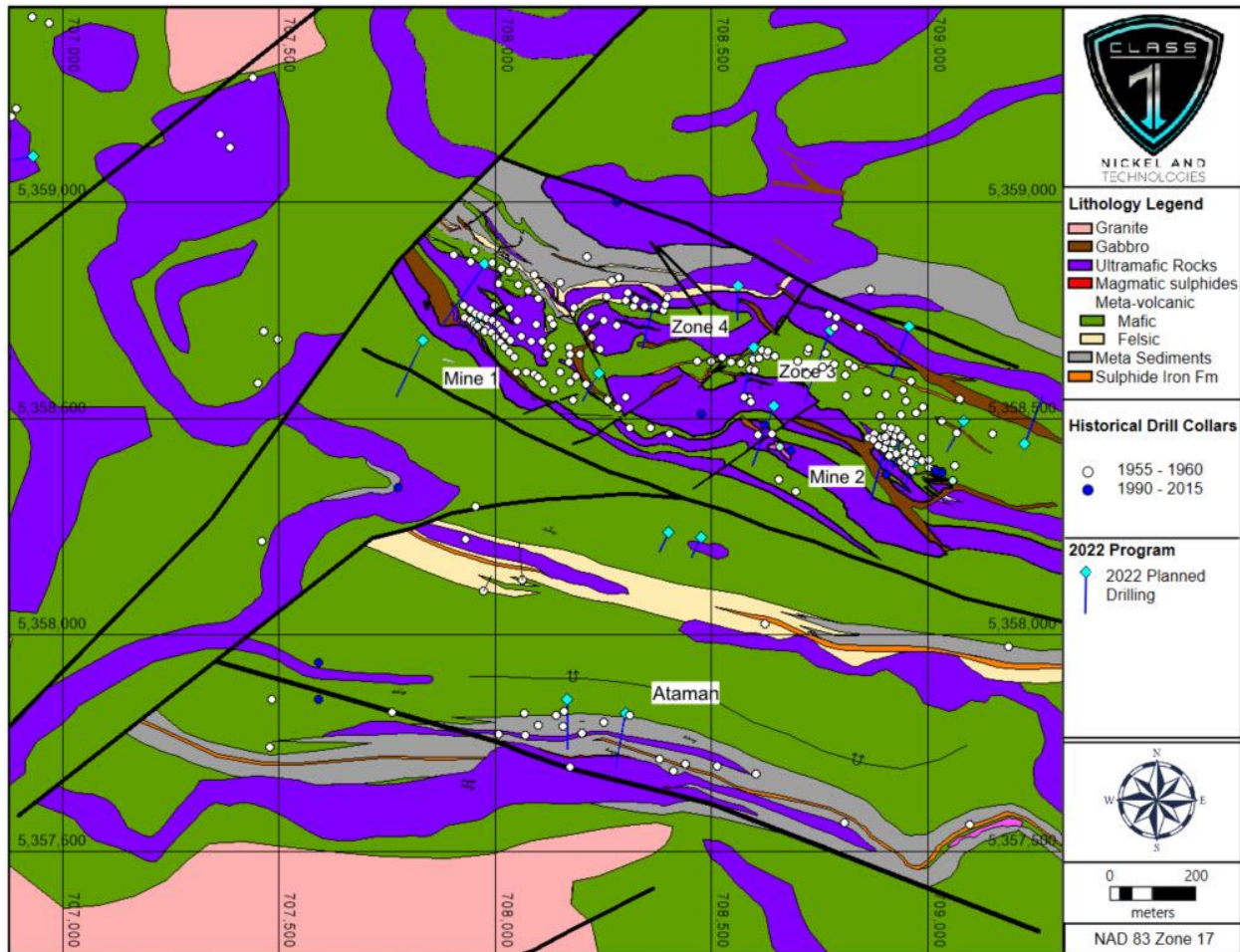
Figure 2: Phase 1 planned drilling
